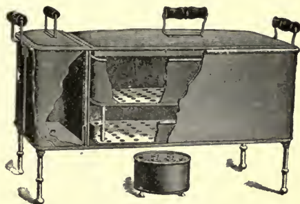
FIG. 161.—A portable sterilizer for dressings and instruments.
